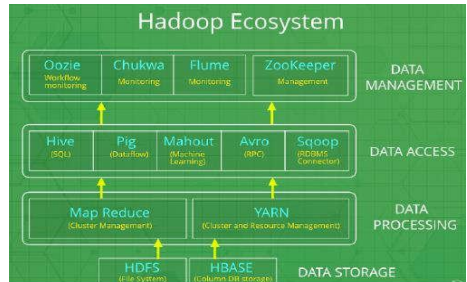
Figure 2.5 Hadoop Ecosystem
