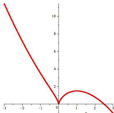
Figure 6.14: y = x^{2/3}(\frac{5}{2} - x)
