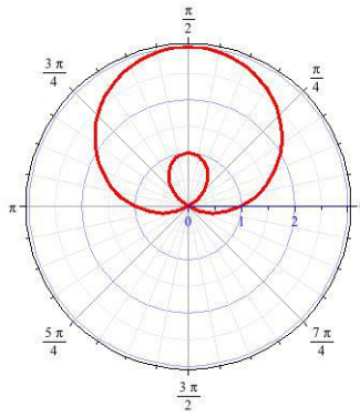
Figure 6.45: r(\theta) = 1 + 2 \sin \theta
