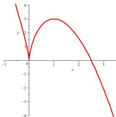
Figure 6.22: f(x) = (5-2x)x^{\frac{2}{3}}
