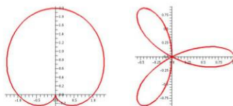
Figure 6.38: r = 1 + \sin \theta and r = \cos 3\theta
