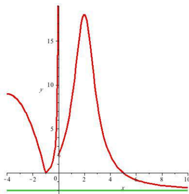
Figure 6.26: Discontinuity at x = 0
