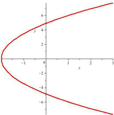
Figure 6.50: y^2 = 24 - 12x
