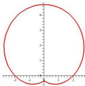
Figure 6.44: r(\theta) = 1 + \sin \theta + e^{\sin \theta}
