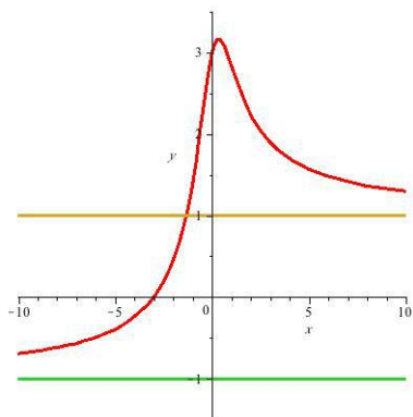
Figure 6.21: f(x) = \frac{x+3}{\sqrt{x^2+1}}
