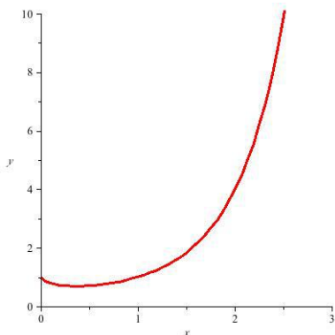
Figure 6.15: y = x^x
