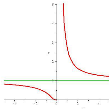
Figure 6.19: f(x) = e^{\frac{1}{x}}
